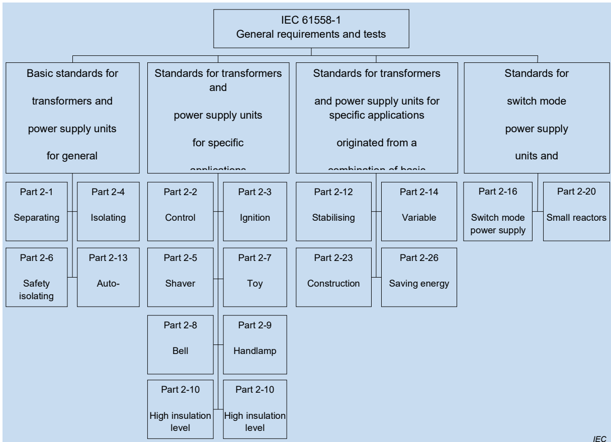
Figure 1 – IEC 61558 principle
